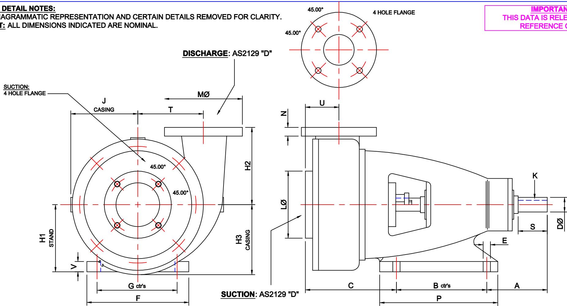
PUMP DIMENSIONS
