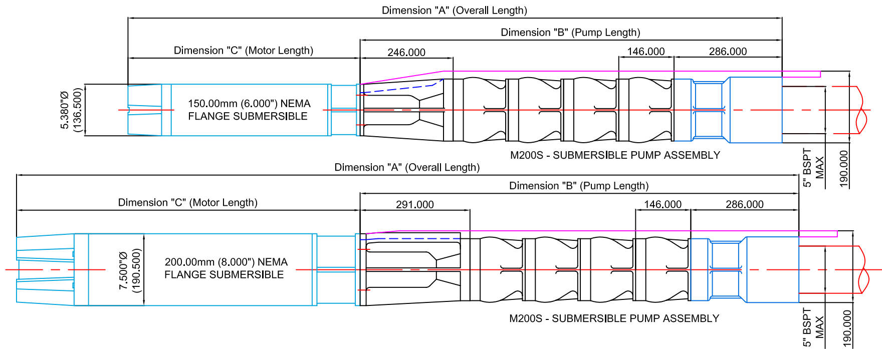
Dimensions (mm) Pump Type - M200S Vertical Series Submersible
