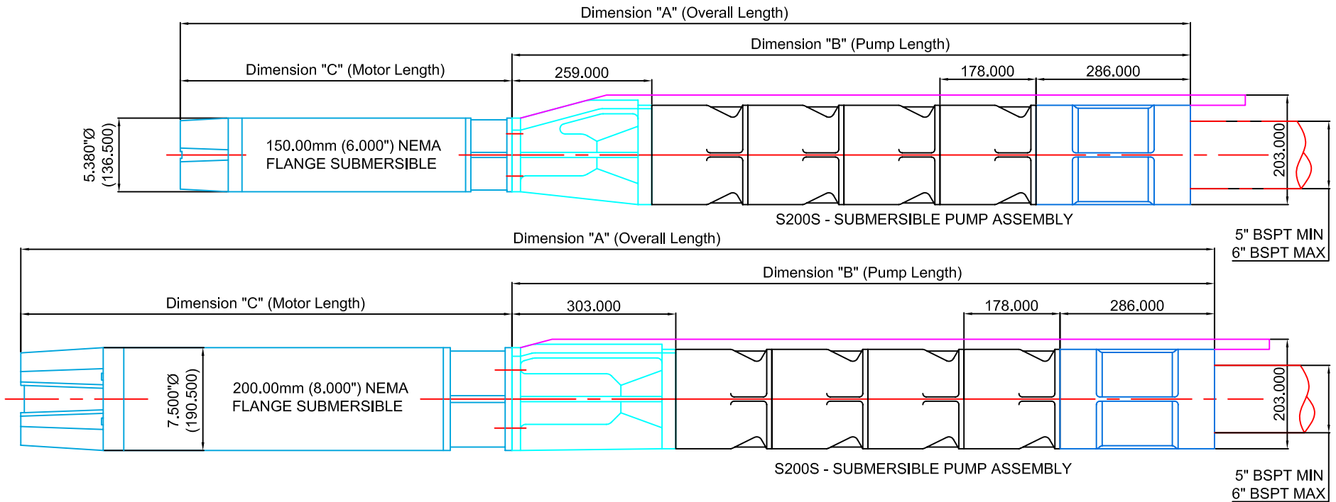
Dimensions (mm) Pump Type - S200S Vertical Series Submersible - 6" and 8" Motors
