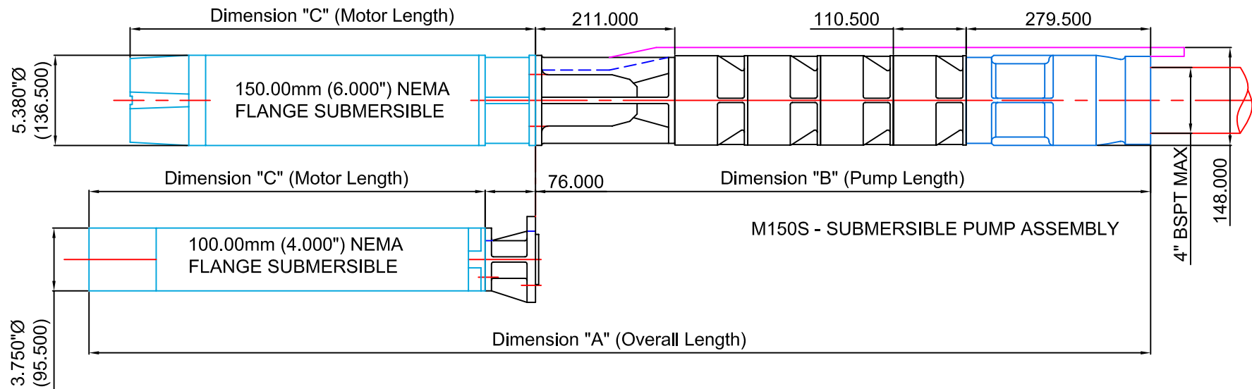
Dimensions (mm) Pump Type - M 150S Vertical Series Submersible
